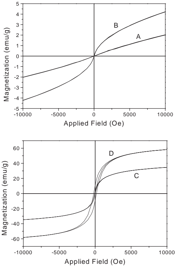
Fig. 5. Magnetization curves versus magnetic field for CoFe 2 O 4 nanoparticles prepared at various temperatures: 20°C (A), 40°C (B), 60°C (C) and 80°C (D).
