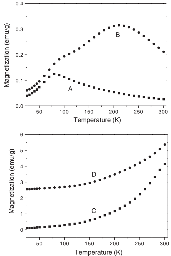
Fig. 6. Temperature dependence of zero-field cooled magnetization of CoFe 2 O 4 nanoparticles prepared at various temperatures: 20°C (A), 40°C (B), 60°C (C) and 80°C (D).
