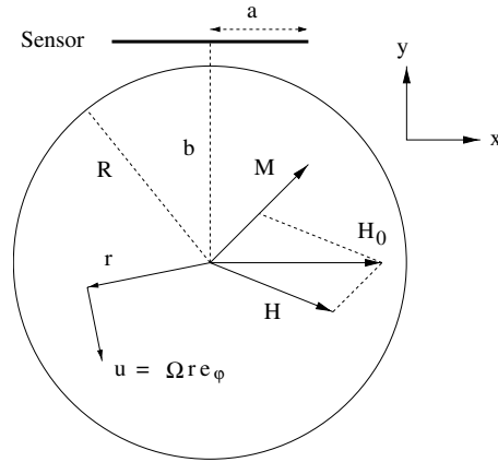
Figure 3. Schematic plot of the system. The cylindrical sample holder with inner radius R rotates with angular velocity \Omega in the applied static magnetic field \mathbf{H}_0 perpendicular to \Omega . The magnetization M_y is measured with a Hall sensor. \mathbf{M} and \mathbf{H} denote the magnetization and internal magnetic field of the ferrofluid. Both are constant in space and time.
