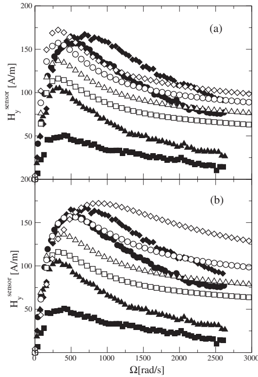
Figure 6. H_y^{\text{sensor}} as a function of \Omega for H_0 = 8.6 \text{ kA m}^{-1} (squares), 15 \text{ kA m}^{-1} (triangles), 30 \text{ kA m}^{-1} (circles), and 60 \text{ kA m}^{-1} (diamonds). Full symbols denote experimental data. Open symbols refer to the polydisperse model (equations (4.1)–(4.3)) with log-normal distribution and K = 15 \text{ kJ m}^{-3} : in (a) the relaxation times \tau_j are independent of H ; in (b) they are replaced by \tau_j^\gamma(H) (5.1) with \gamma = 10^{-4} \text{ m A}^{-1} .
